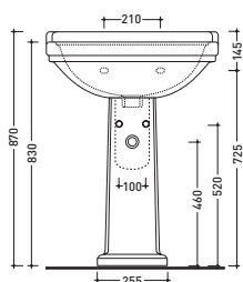
vista frontale / frontal view
