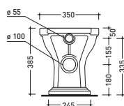
vista retro / back view
