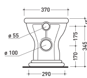
vista retro / back view
