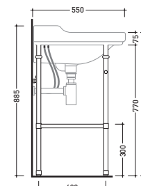
vista laterale / lateral view
